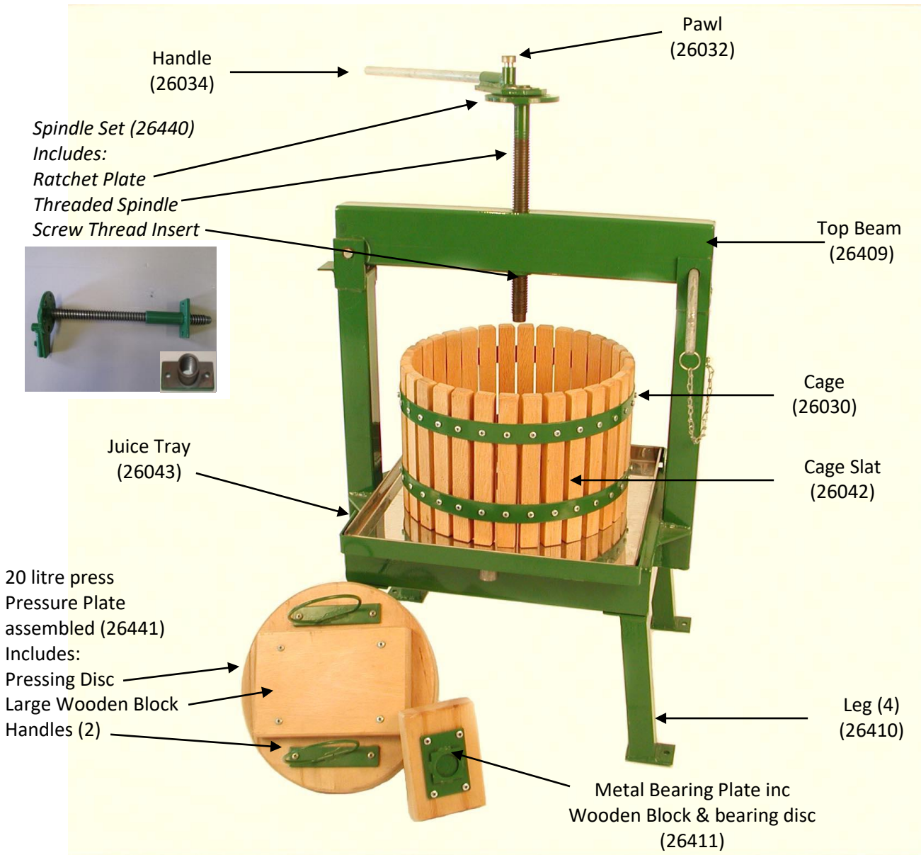
Bearing Disc (26412)
